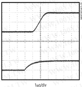
MAX5383 OUTPUT SETTLING FROM 1/4FS TO 3/4FS
