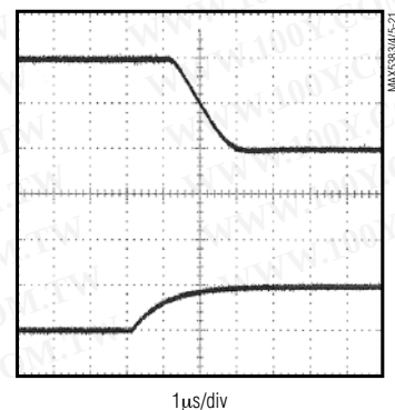
MAX5383 OUTPUT SETTLING FROM 3/4FS TO 1/4FS
