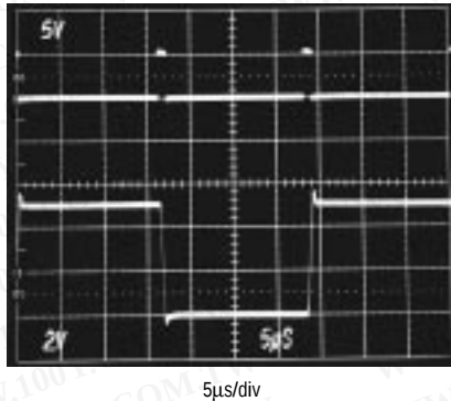
MAX536 DYNAMIC RESPONSE (ALL BITS ON, OFF, ON)
