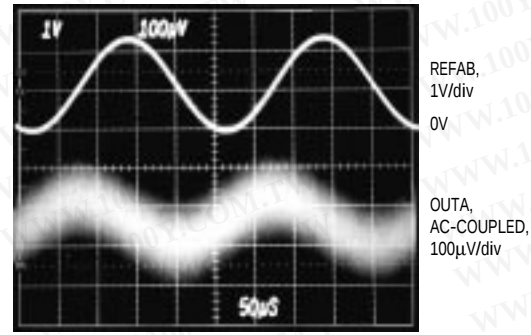
MAX537 REFERENCE FEEDTHROUGH AT 4kHz
