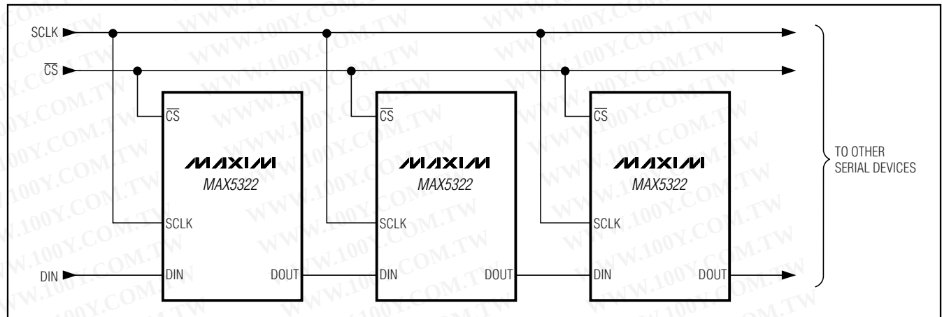
Figure 7. Daisy-Chaining Devices
