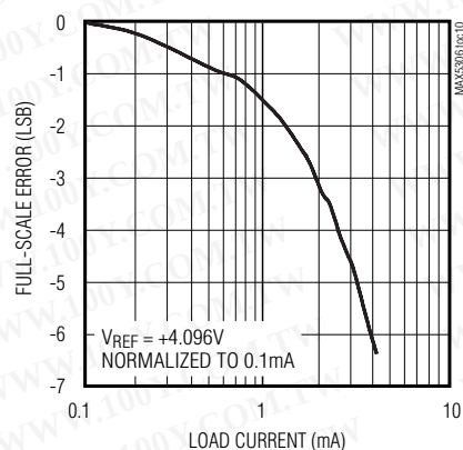
FULL-SCALE ERROR vs. LOAD CURRENT
