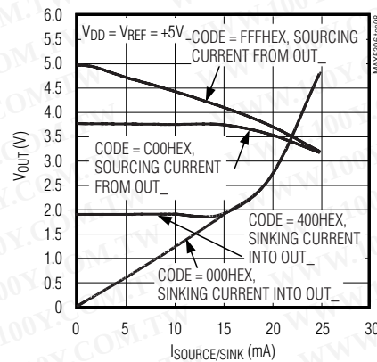
SOURCE-AND-SINK CURRENT CAPABILITY
