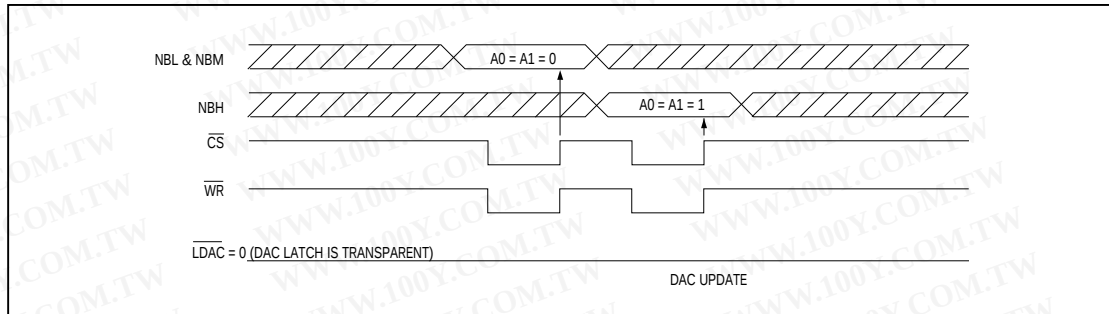
Figure 8b. 8-Bit and 16-Bit \mu P Timing Sequence with \overline{\text{LDAC}} = 0
