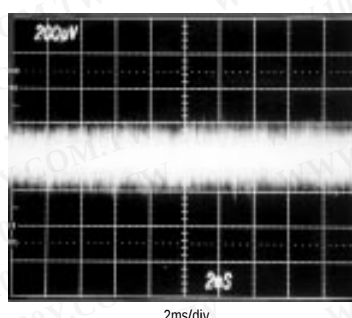
OUTPUT VOLTAGE NOISE (DC TO 1MHz)
