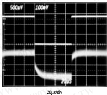
LINE-TRANSIENT RESPONSE (OUTA)
