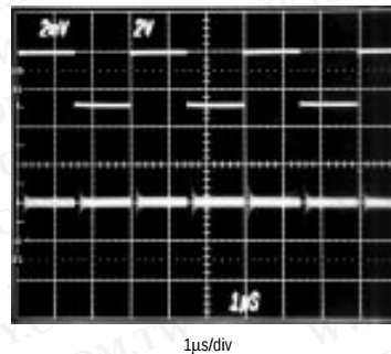
CLOCK FEEDTHROUGH (OUTA)
