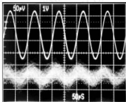
REFERENCE FEEDTHROUGH AT 10kHz
