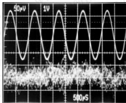
REFERENCE FEEDTHROUGH AT 1kHz
