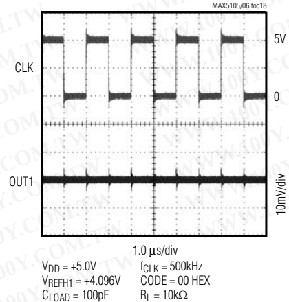
CLOCK FEEDTHROUGH
