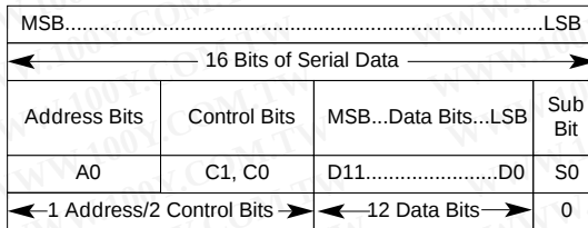
Figure 4. Serial-Data Format
