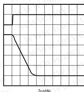
DYNAMIC RESPONSE FALL TIME
