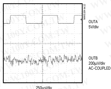
ANALOG CROSSTALK
