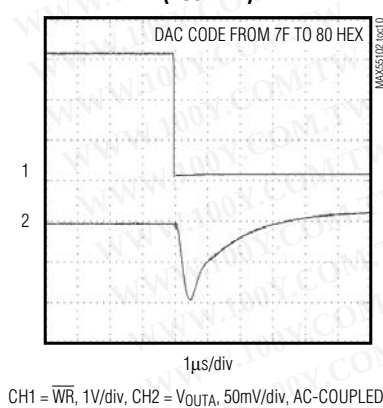
WORST-CASE 1LSB DIGITAL STEP CHANGE (POSITIVE)
