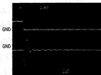
DIGITAL FEEDTHROUGH – GLITCH IMPULSE (1 TO 0 DIGITAL TRANSITION)
