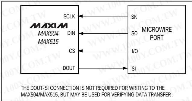
Figure 4. Microwire Connection
