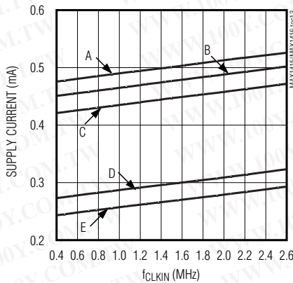
SUPPLY CURRENT vs. f_{CLKIN} (MAX1415)
