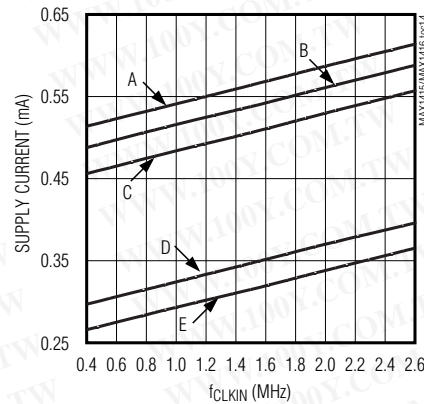
SUPPLY CURRENT vs. f_{CLKIN} (MAX1416)
