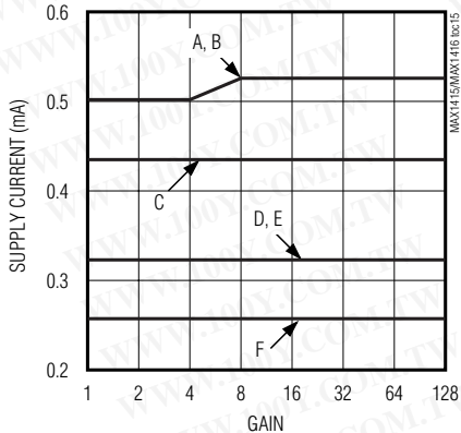
SUPPLY CURRENT vs. GAIN (MAX1415)
