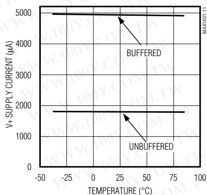
V_+ SUPPLY CURRENT vs. TEMPERATURE (240sps OUTPUT DATA RATE)
