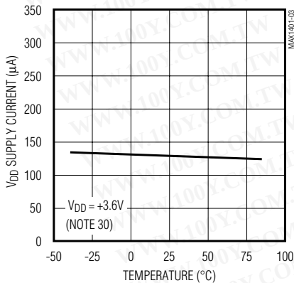
V_{DD} SUPPLY CURRENT vs. TEMPERATURE (20sps OUTPUT DATA RATE UNBUFFERED)
