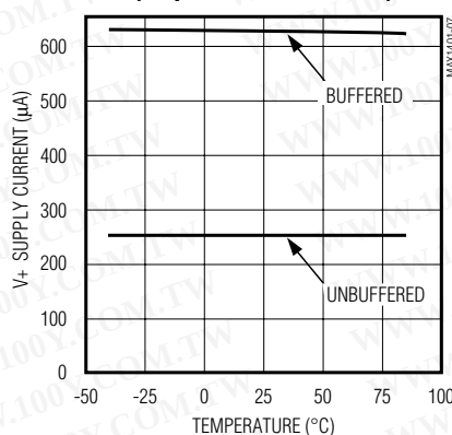
V_+ SUPPLY CURRENT vs. TEMPERATURE (60sps OUTPUT DATA RATE)
