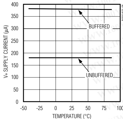
V_+ SUPPLY CURRENT vs. TEMPERATURE (20sps OUTPUT DATA RATE)
