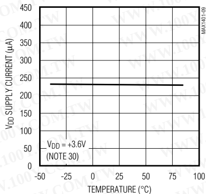
V_{DD} SUPPLY CURRENT vs. TEMPERATURE (240sps OUTPUT DATA RATE UNBUFFERED)
