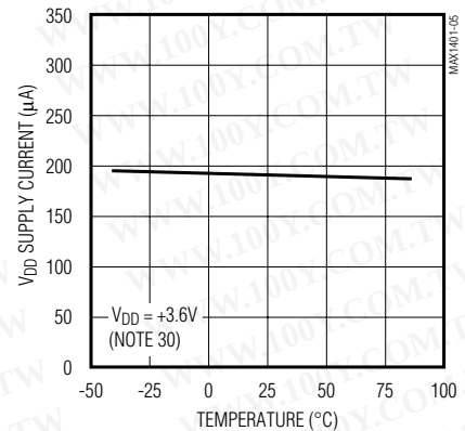
V_{DD} SUPPLY CURRENT vs. TEMPERATURE (120sps OUTPUT DATA RATE UNBUFFERED)
