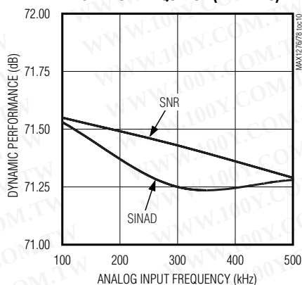
DYNAMIC PERFORMANCE vs. INPUT FREQUENCY (MAX1278)
