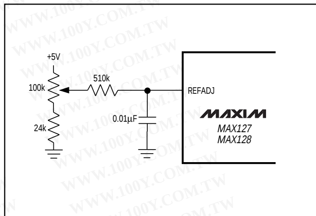
Figure 12. Reference-Adjust Circuit
