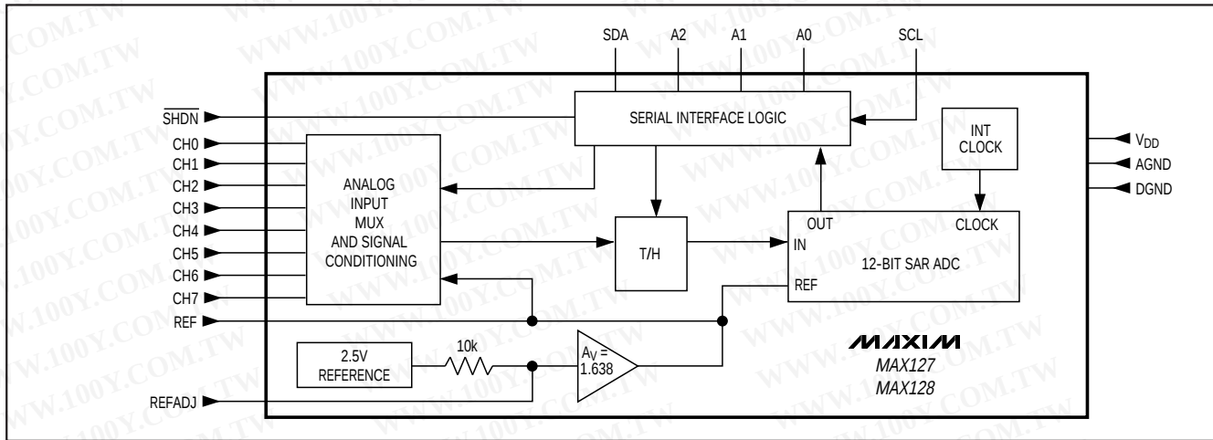
Figure 1. Block Diagram
