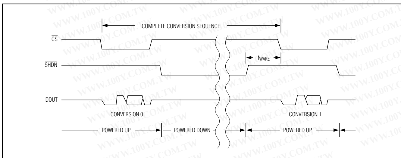
Figure 5. Shutdown Sequence
