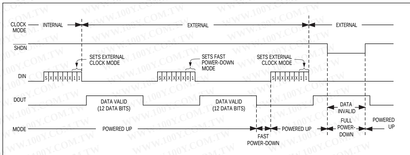
Figure 12a. Timing Diagram for Power-Down Modes, External Clock
