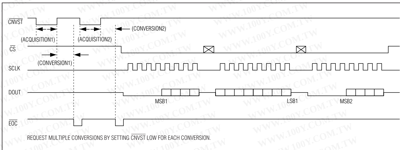
Figure 5. Clock Mode 01 Timing
