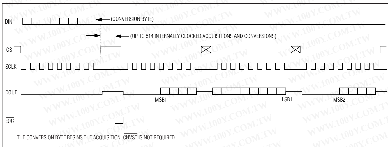
Figure 6. Clock Mode 10 Timing
