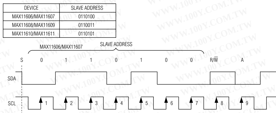
Figure 7. MAX11606/MAX11607 Slave Address Byte
