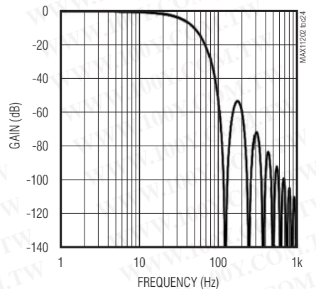
NORMAL MODE REJECTION OF 50Hz TO 60Hz (MAX11202B)
