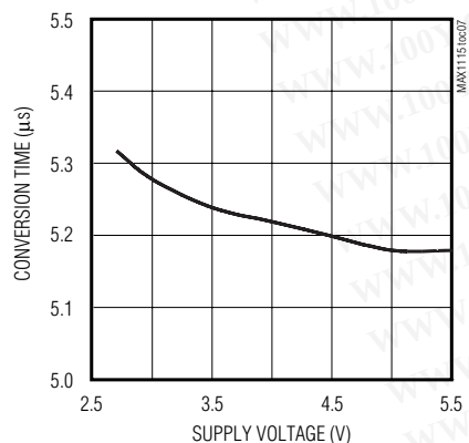
CONVERSION TIME vs. SUPPLY VOLTAGE
