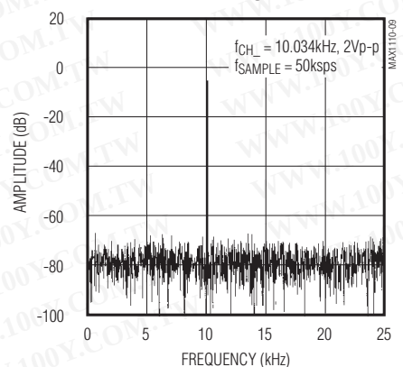
FFT PLOT
