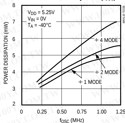
MAX110 POWER DISSIPATION vs. OVERSAMPLING FREQUENCY ( f_{OSC} )
