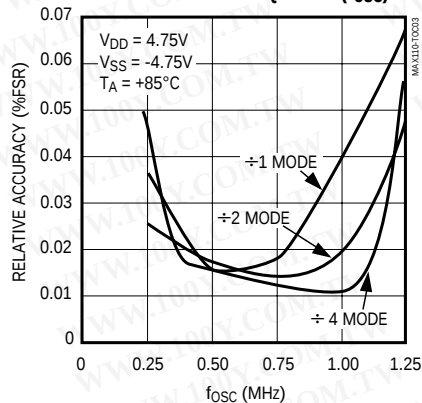
MAX110 RELATIVE ACCURACY vs. OVERSAMPLING FREQUENCY ( f_{OSC} )
