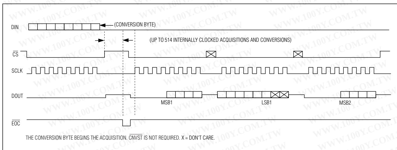
Figure 6. Clock Mode 10
