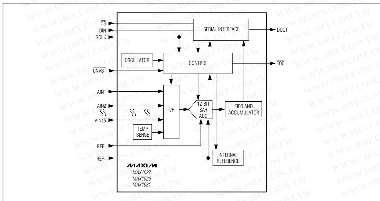
Figure 2. Functional Diagram
