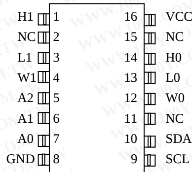
DS1803Z 16-PIN SO (150 MIL)
