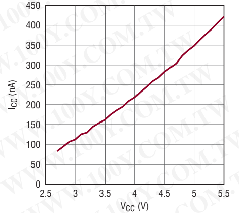
I_{CC} Shutdown vs V_{CC}
