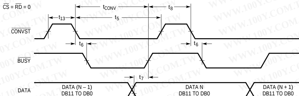
Figure 15. Mode 1b. \overline{\text{CONVST}} Starts a Conversion. Data Outputs Always Enabled ( \overline{\text{CONVST}} = \text{[Pulse]} )
