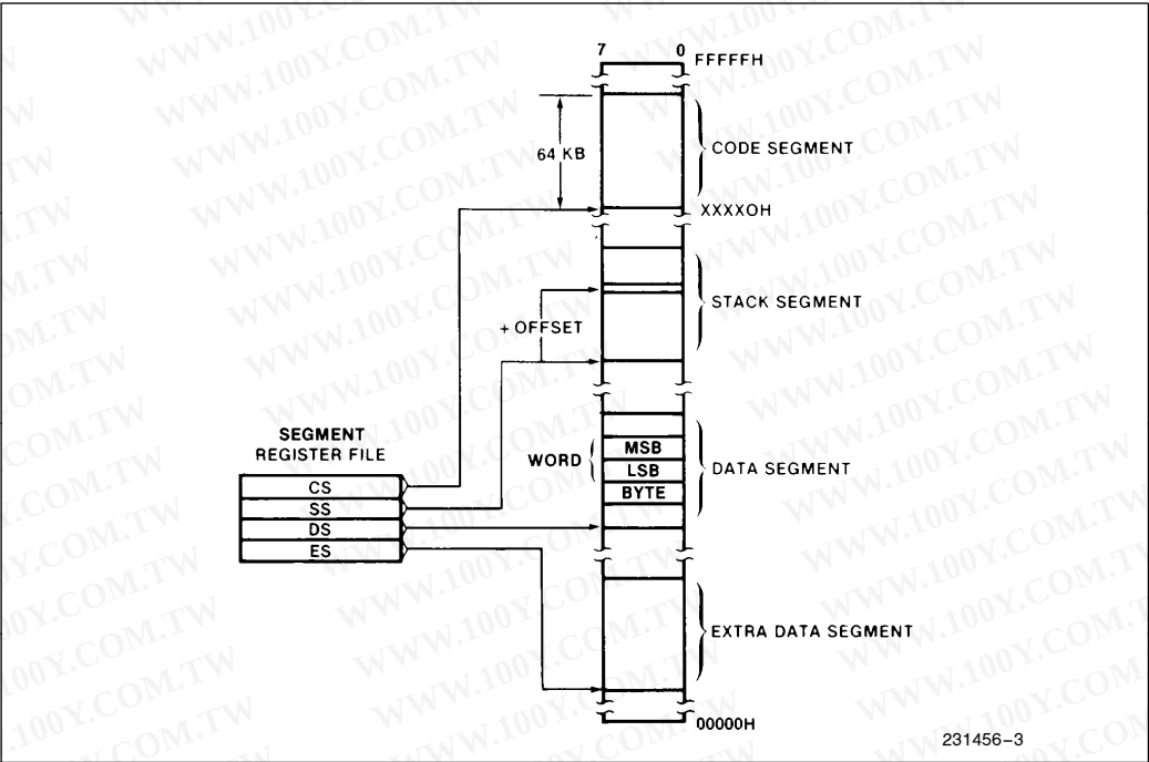
Figure 3. Memory Organization
