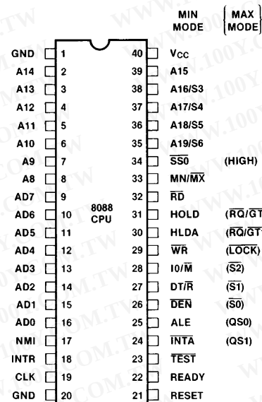
Figure 2. 8088 Pin Configuration
