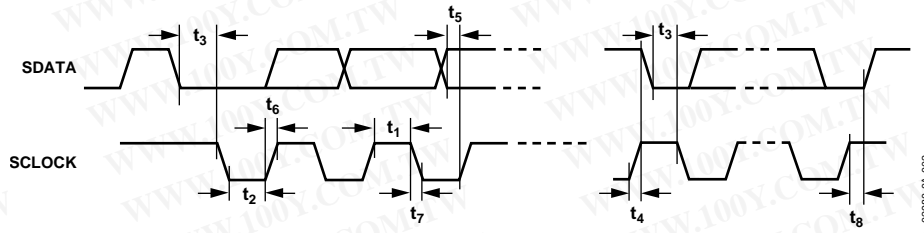
Figure 2. MPU Port Timing Diagram
