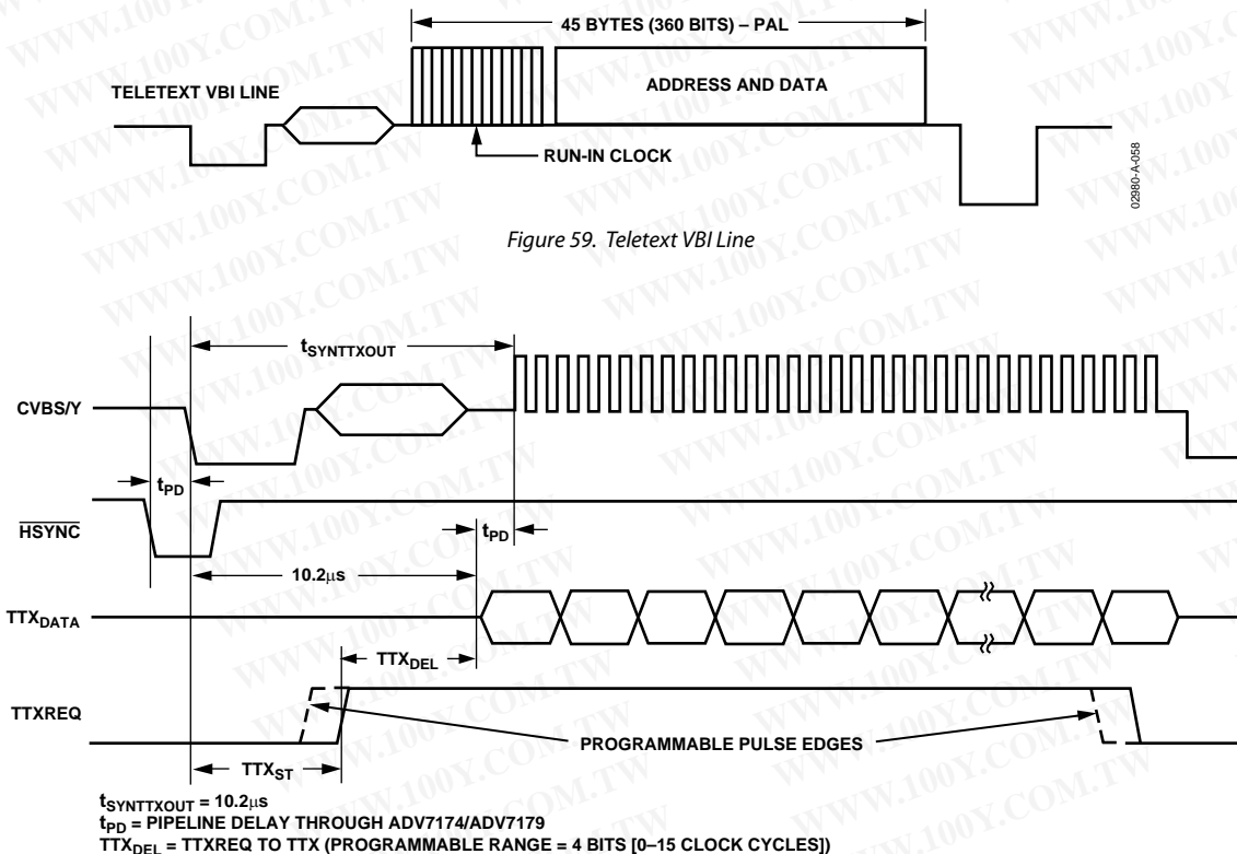
Figure 60. Teletext Functionality
