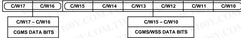
Figure 52. CGMS_WSS Register 1
