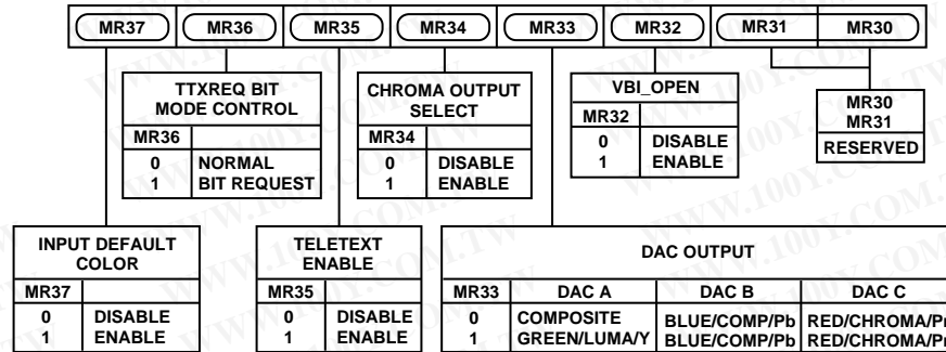
Figure 41. Mode Register 3
