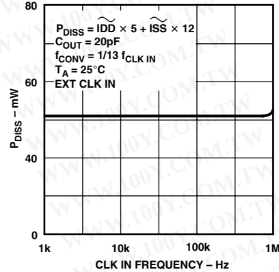
TPC 5. Power Dissipation vs. CLK IN Frequency
