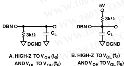
Figure 3. Load Circuits for Access Time
