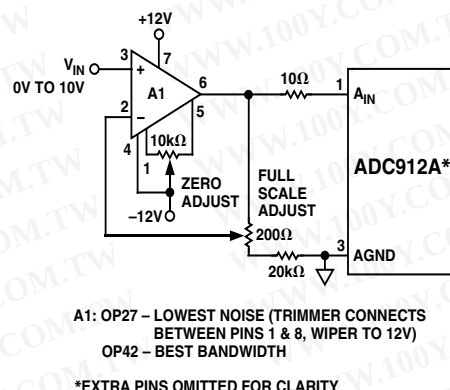
Figure 16. Unipolar 0 V to 10 V Operation
