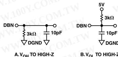
Figure 4. Load Circuits for Output Float Delay
