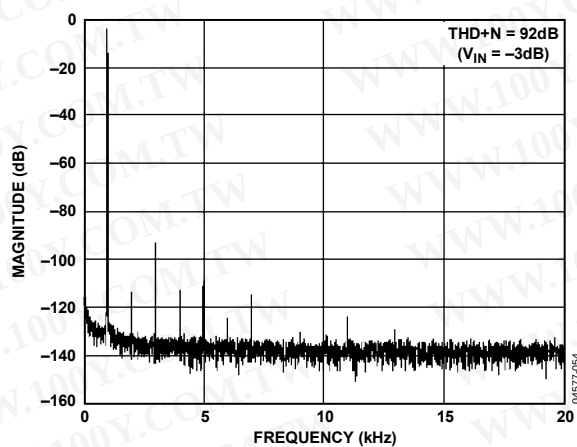
Figure 20. DAC THD + N, f_s = 48 kHz
