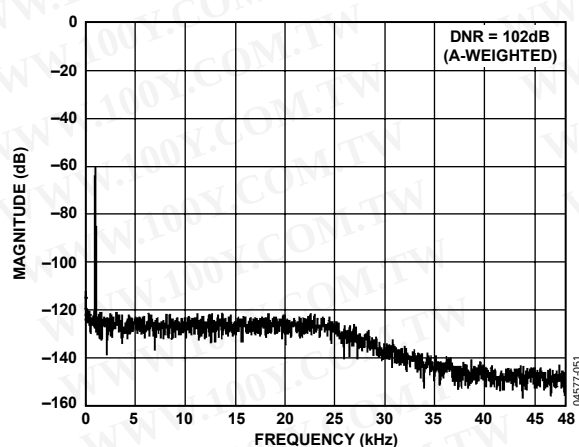
Figure 17. DAC Dynamic Range, f_s = 96 kHz
