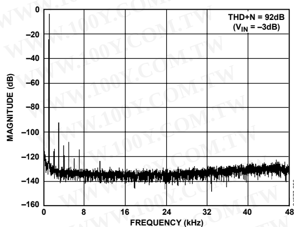
Figure 22. ADC THD + N, f_s = 96 kHz
