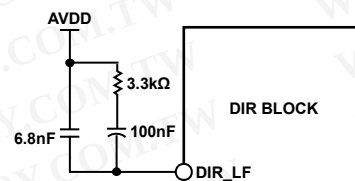
Figure 42. DIR Loop Filter Components
