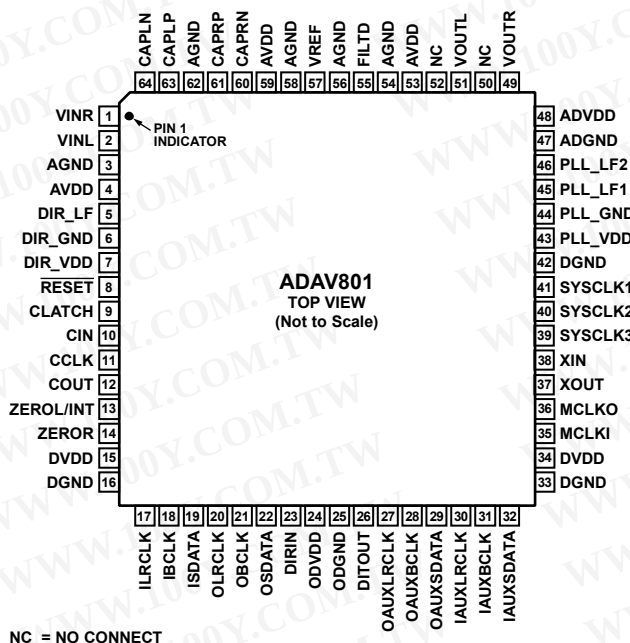
Figure 2. ADAV801 Pin Configuration
