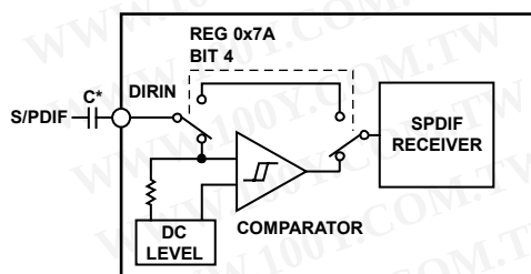
Figure 39. DIRIN Block
