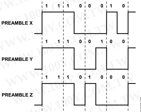
Figure 45. Preambles
