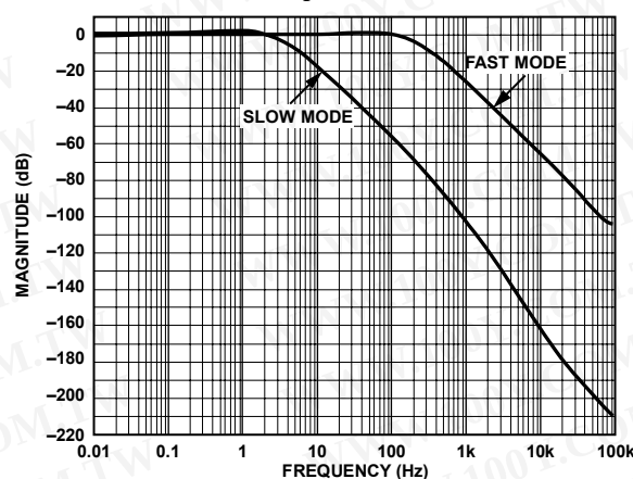
Figure 34. Frequency Response of the Digital Servo Loop; f_{S\_IN} is the X-Axis, f_{S\_OUT} = 192 kHz, Master Clock is 30 MHz
