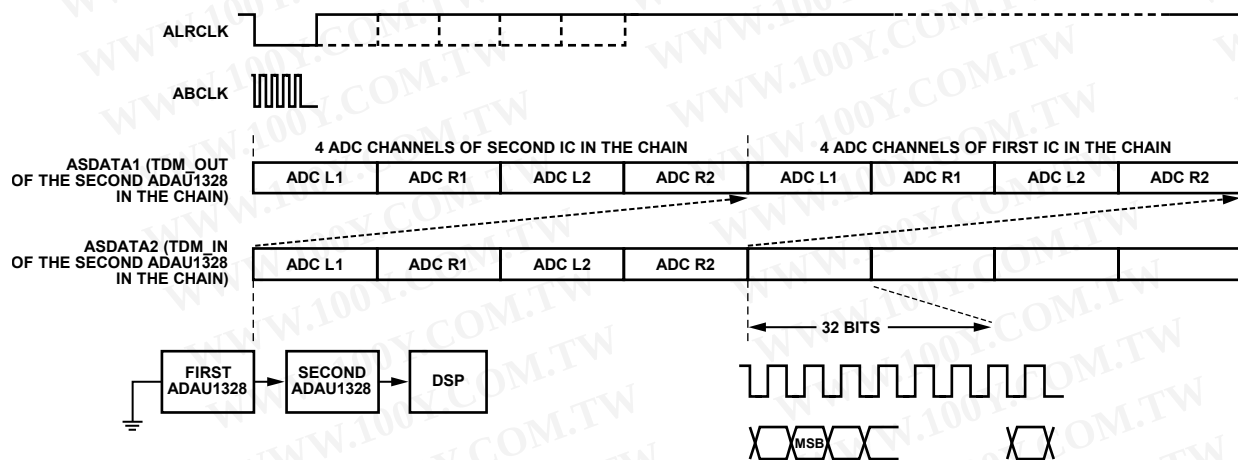
Figure 21. Dual-Line ADC TDM Daisy-Chain Mode (256 fs ABCLK, Two ADAU1328 Daisy Chain)
