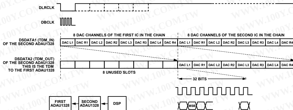
Figure 18. Single-Line DAC TDM Daisy-Chain Mode (Applicable to 48 kHz Sample Rate, 16-Channel, Two ADAU1328 Daisy Chain)
