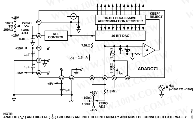
Figure 12. Analog and Power Connections for Bipolar -10\text{ V} to +10\text{ V} Input Range
