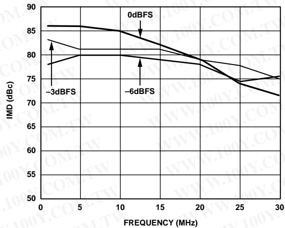
Figure 16. Third-Order IMD Products vs. Two-Tone f_{OUT} @ f_{DATA} = 78 MSPS
