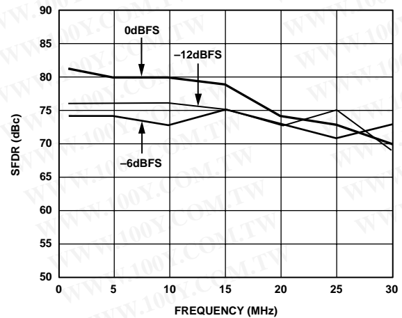
Figure 11. Out-of-Band SFDR vs. f_{OUT} @ f_{DATA} = 78\text{ MSPS}
