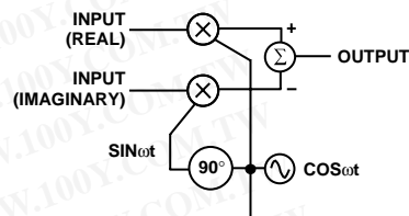
Figure 78. Quadrature Modulation
