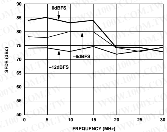
Figure 10. In-Band SFDR vs. f_{OUT} @ f_{DATA} = 78\text{ MSPS}
