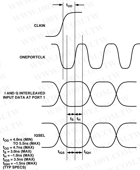
Figure 56. Timing Requirements in One-Port Input Mode, with PLL Disabled
