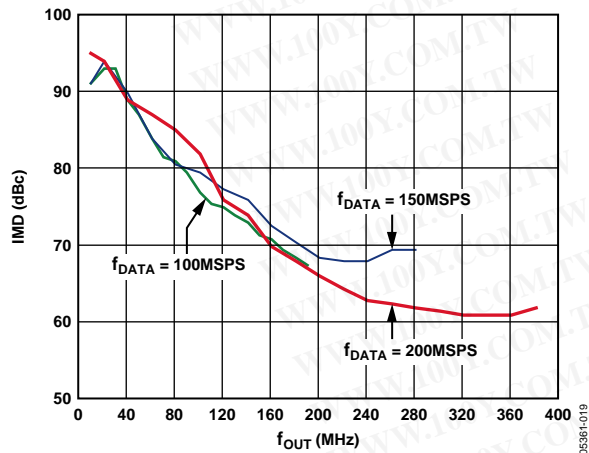
Figure 20. AD9779 Third-Order IMD vs. f_{OUT} , 4x Interpolation
