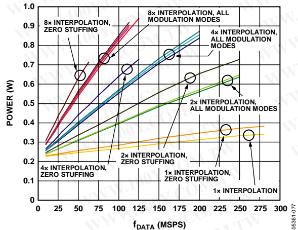
Figure 85. Total Power Dissipation, Dual DAC Mode
