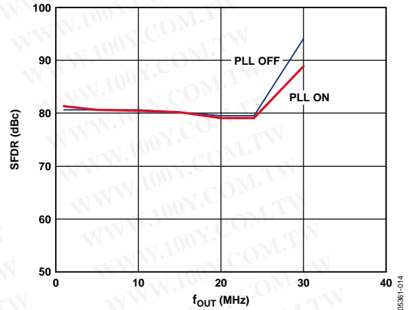
Figure 15. AD9779 In-Band SFDR, 4x Interpolation, f_{DATA} = 100MSPS , PLL On/Off
