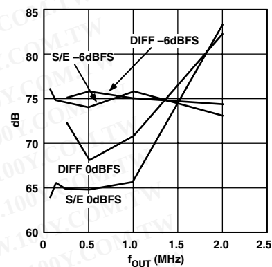
TPC 12. SFDR vs. f_{\text{OUT}} (DC to f_{\text{DATA}}/2 )
