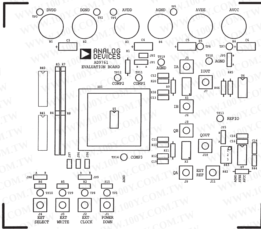
Figure 25. Silkscreen Layer—Top
