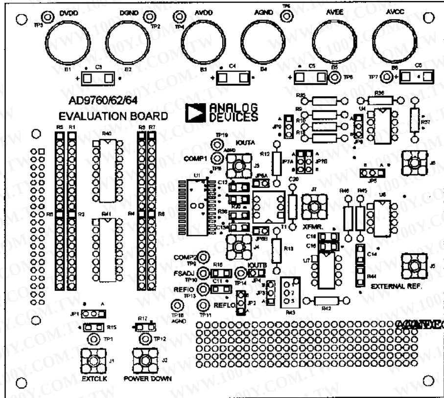
Figure 42. Silkscreen Layer—Top
