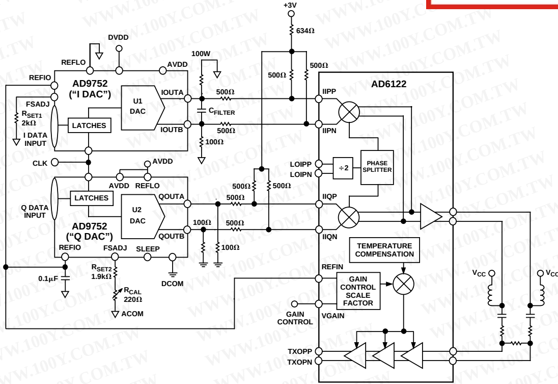
Figure 38. CDMA Transmit Application Using AD9752
