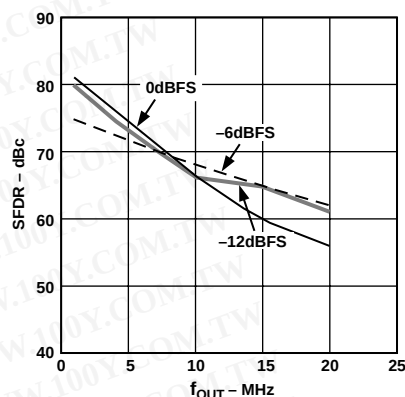
Figure 5. SFDR vs. f_{OUT} @ 50 MSPS
