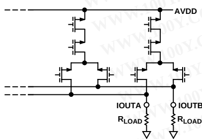
Figure 22. Equivalent Analog Output
