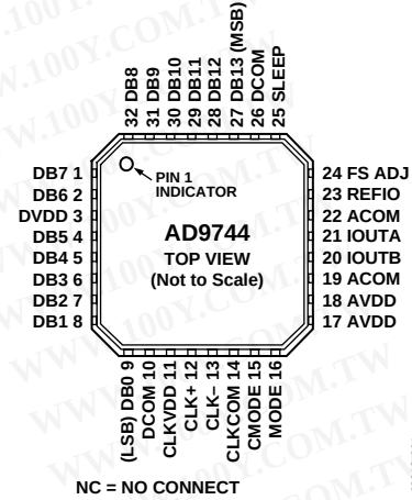
Figure 4. 32-Lead LFCSP
