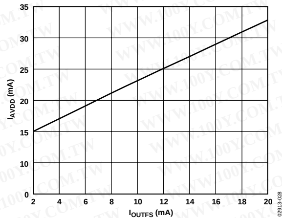
Figure 31. I_{AVDD} vs. I_{OUTFS}
