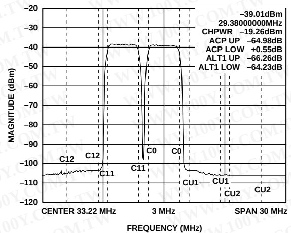
Figure 22. Two-Carrier UMTS Spectrum, f_{\text{CLOCK}} = 122.88 \text{ MSPS} (ACLR = 64 dB) LFCSP Package
