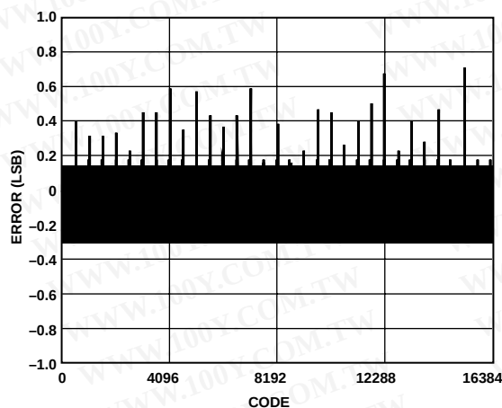
Figure 17. Typical DNL
