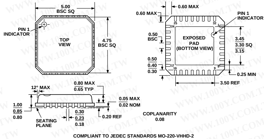
Figure 60. 32-Lead Frame Chip Scale Package [LFCSP] 5 mm x 5 mm Body (CP-32-3) Dimensions shown in millimeters
