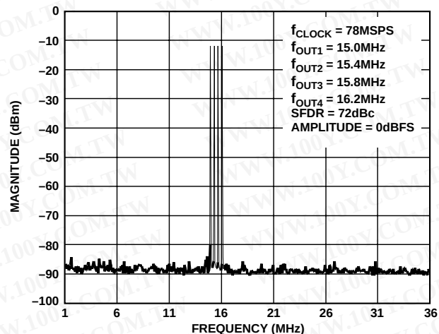
Figure 21. Four-Tone SFDR
