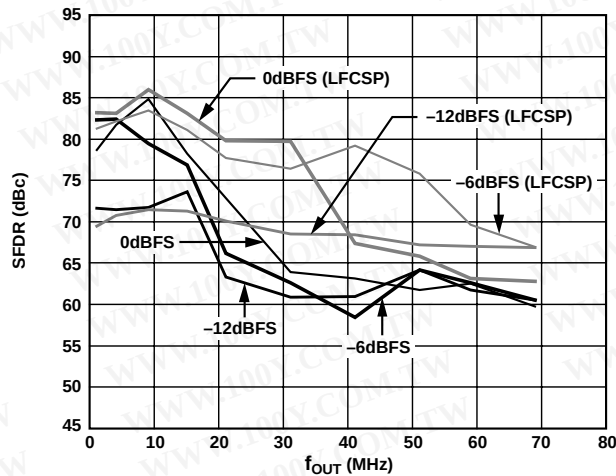
Figure 11. SFDR vs. f_{OUT} @ 210 MSPS
