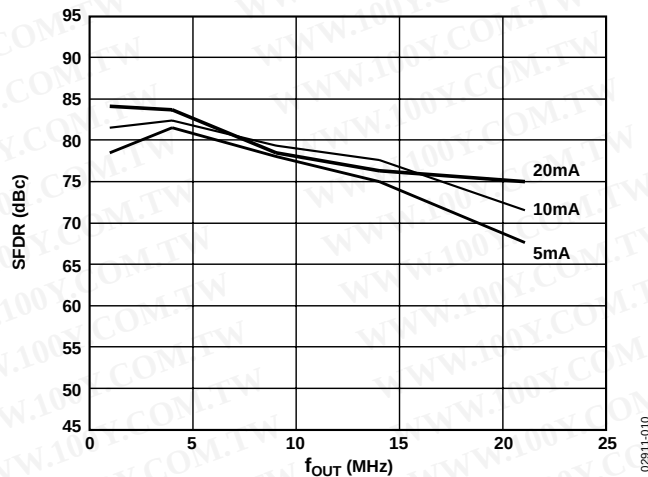
Figure 10. SFDR vs. f_{OUT} and I_{OUTS} @ 65 MSPS and 0 dBFS
