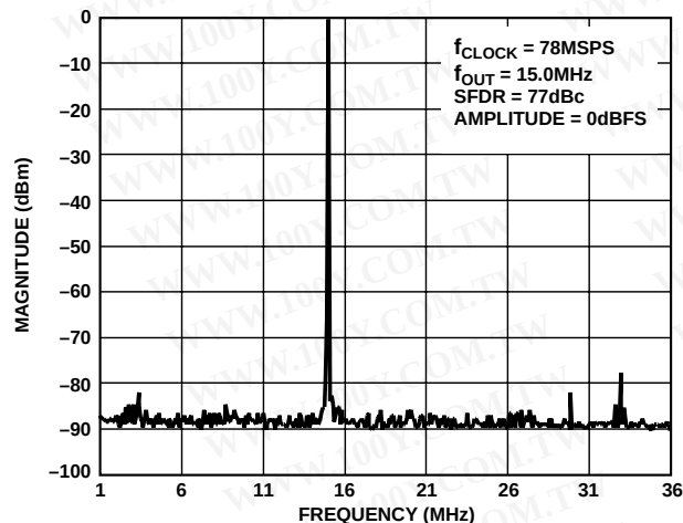
Figure 19. Single-Tone SFDR
