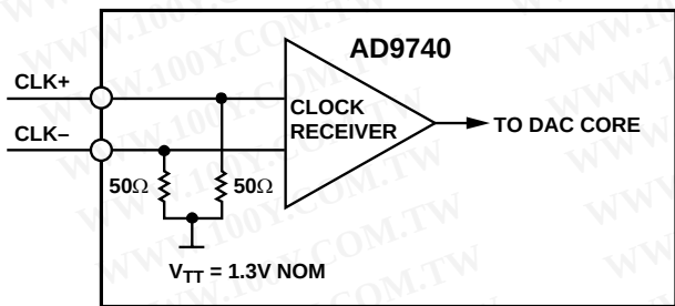
Figure 27. Clock Termination in PECL Mode
