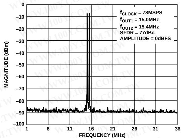
Figure 20. Dual-Tone SFDR
