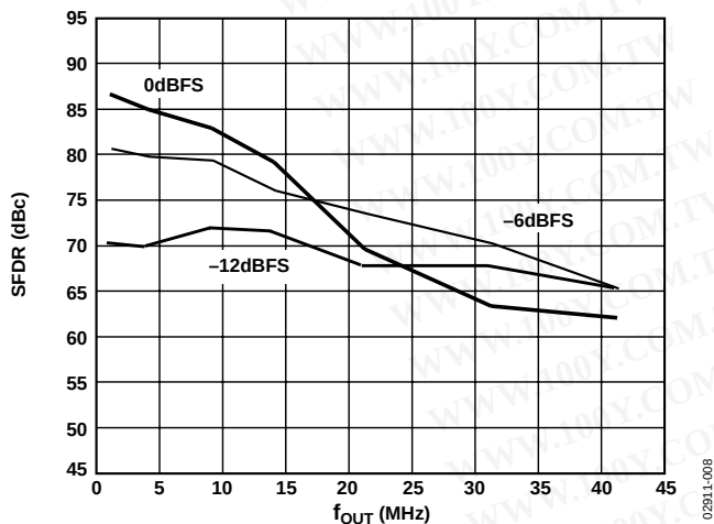
Figure 8. SFDR vs. f_{OUT} @ 125 MSPS
