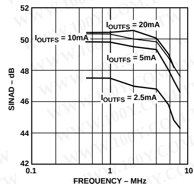
Figure 8. SINAD vs. I_{OUTFS} @ 20 MSPS
