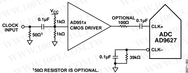
150Ω RESISTOR IS OPTIONAL. Figure 60. Single-Ended 1.8 V CMOS Sample Clock (Up to 150 MSPS)
