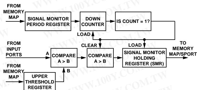
Figure 70. ADC Input Threshold Crossing Block Diagram
