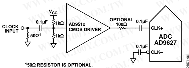
150Ω RESISTOR IS OPTIONAL. Figure 61. Single-Ended 3.3 V CMOS Sample Clock (Up to 150 MSPS)
