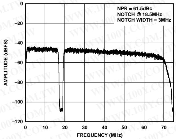
Figure 38. AD9627-150 Noise Power Ratio (NPR)
