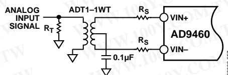
Figure 47. Transformer-Coupled Analog Input Circuit
