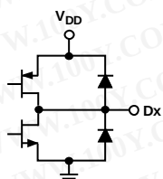
Figure 38. Digital Output Circuit
