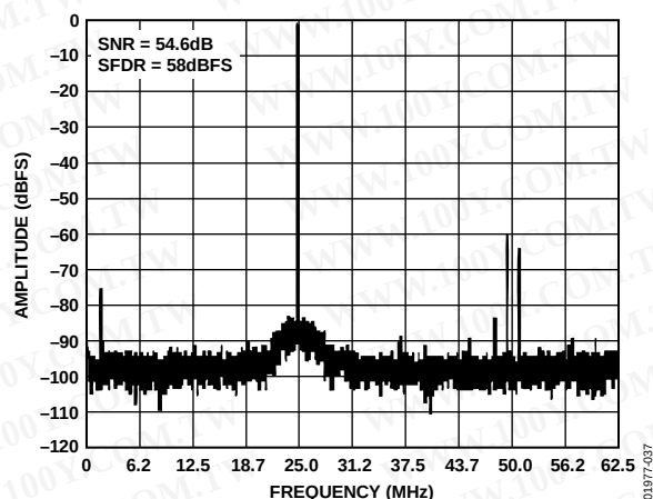
Figure 32. FFT: f_s = 125 MSPS, f_{IN} = 350.3 MHz, Differential AIN @ -0.5 dBFS, SFDR Mode Enabled
