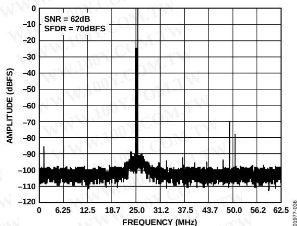
Figure 31. FFT: f_s = 125 MSPS, f_{IN} = 150.3 MHz, Differential AIN @ -0.5 dBFS, SFDR Mode Enabled
