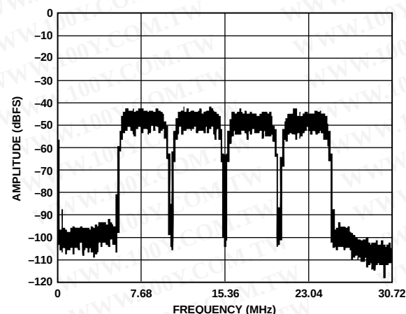
Figure 21. FFT: f_s = 61.44 MSPS, f_{IN} = 46.08 MHz, Four WCDMA Carriers, Differential AIN, SFDR Mode Enabled
