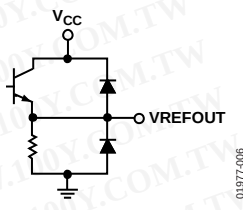
Figure 39. Voltage Reference Output Circuit
