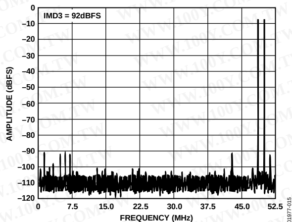
Figure 10. FFT: f_s = 105 MSPS, f_{IN} = 49.3 MHz and 50.3 MHz, Differential AIN @ -7 dBFS for Each Tone, SFDR Mode Enabled
