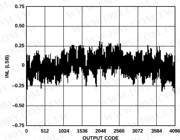
Figure 20. Integral Nonlinearity vs. Output Code with SFDR Mode Enabled
