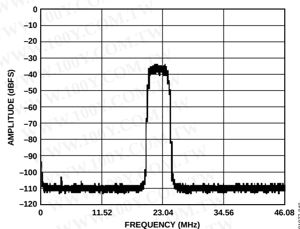
Figure 35. FFT: f_s = 92.16 MSPS, f_{in} = 70.3 MHz, WCDMA @ 70.0 MHz, SFDR Mode Enabled
