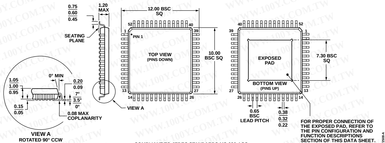
Figure 47. 52-Lead Thin Quad Flat Package, Exposed Pad [TQFP_EP] (SV-52-2) Dimensions shown in millimeters
