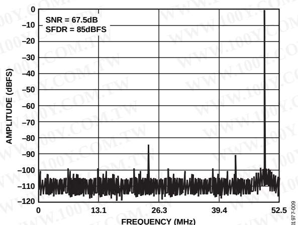
Figure 4. FFT: f_s = 105 MSPS, f_{IN} = 49.3 MHz, Differential AIN @ -0.5 dBFS, SFDR Mode Enabled
