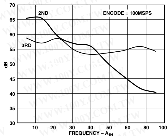
TPC 4. Harmonic Distortion vs. A_{IN} Frequency
