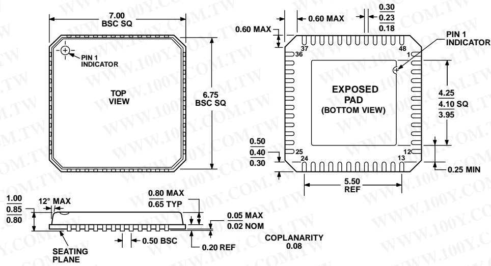
COMPLIANT TO JEDEC STANDARDS MO-220-VKKD-2 Figure 64. 48-Lead Lead Frame Chip Scale Package [LFCSP_VQ] 7 mm × 7 mm Body, Very Thin Quad (CP-48-3) Dimensions shown in millimeters
