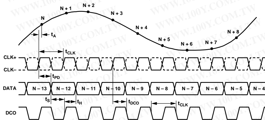
Figure 2. Timing Diagram
