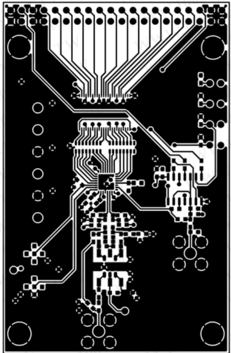
Figure 52. LFCSP Evaluation Board Layout, Primary Side
