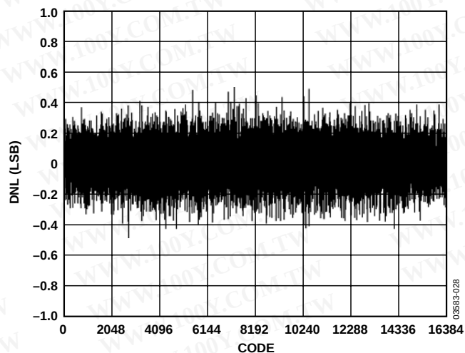
Figure 19. Typical DNL
