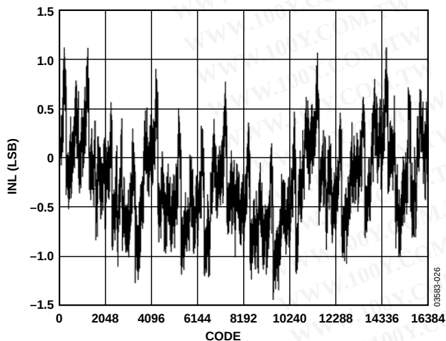
Figure 16. Typical INL
