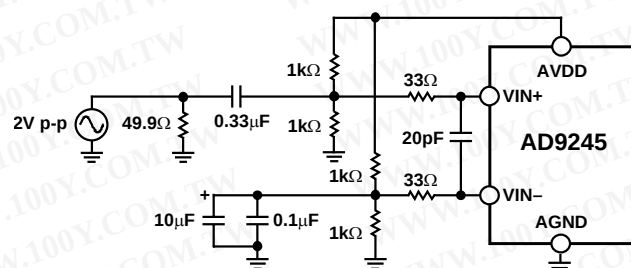
Figure 42. Single-Ended Input Configuration
