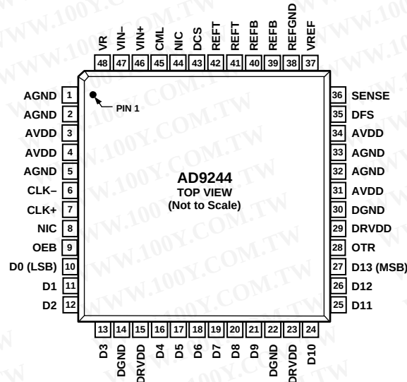
Figure 3. Pin Configuration
