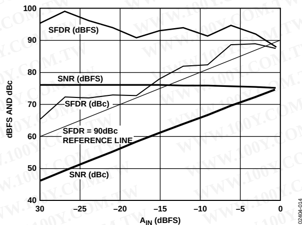
Figure 14. Single-Tone SNR/SFDR vs. A_{\text{IN}} , f_{\text{IN}} = 31 MHz
