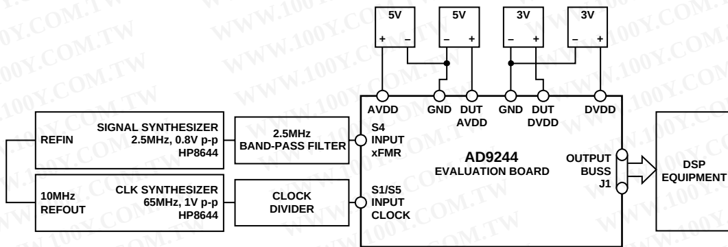
Figure 64. Evaluation Board Connections
