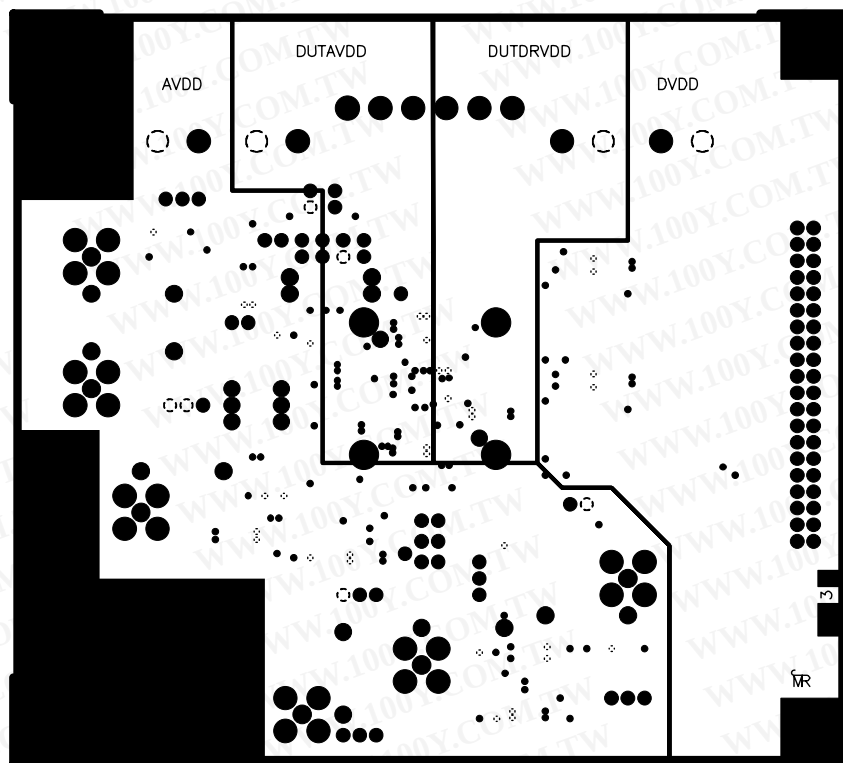
Figure 72. AD9244 Evaluation Board, PCB Layer 3 (Power Plane)
