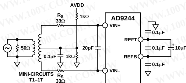
Figure 46. Transformer-Coupled Input
