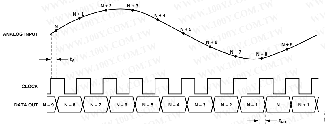
Figure 2. Input Timing
