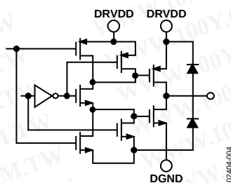
Figure 4. D0 to D13, OTR
