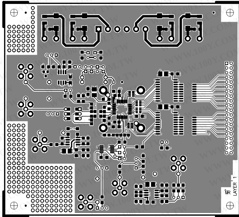
Figure 70. AD9244 Evaluation Board, PCB Layer 1 (Top)
