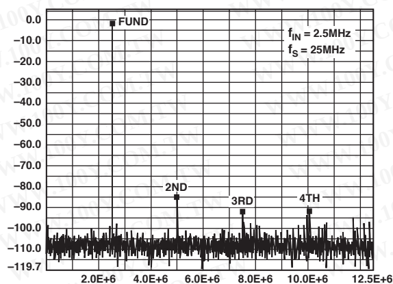
Figure 16. Single-Tone Frequency Domain Plot Common-Mode Voltage = 2.5 V ( A_{IN} = 4\text{ V Differential} )
