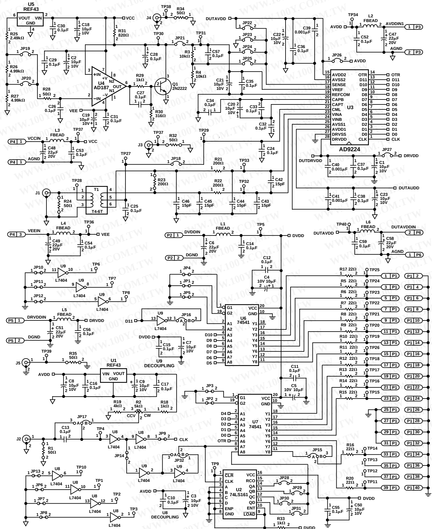
Figure 44. Evaluation Board Schematic
