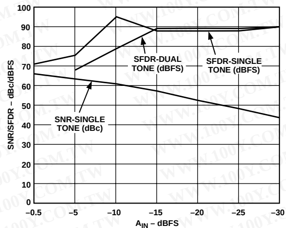
Figure 38. IF Undersampling at 70 MHz ( F_1 = 70.46 MHz, F_2 = 71.36 MHz, f_{\text{CLOCK}} = 31.5 MSPS)
