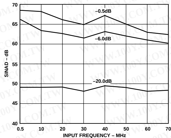
Figure 6. SINAD vs. Input Frequency (Input Span = 2.0 V p-p, V_{CM} = 2.5 V Differential Input)
