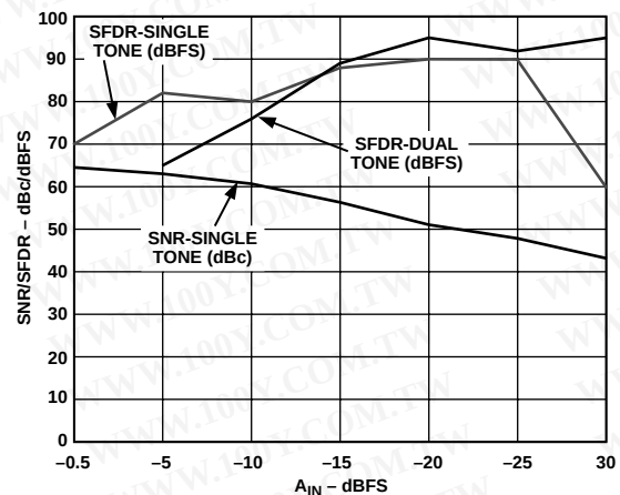
Figure 39. IF Undersampling at 85 MHz ( F_1 = 84.46 MHz, F_2 = 85.36 MHz, f_{\text{CLOCK}} = 31 MSPS)
